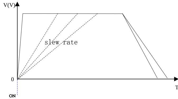
Output voltage, current up/down slew rate
